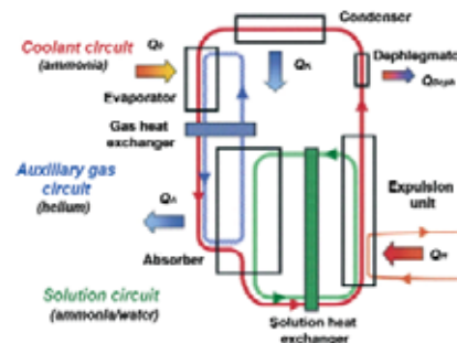
Single-stage continuous absorption cooling system
